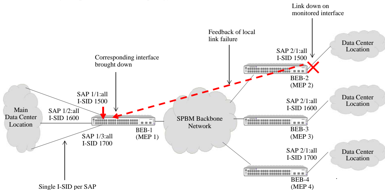
Figure 10: RFP for SPB Example
