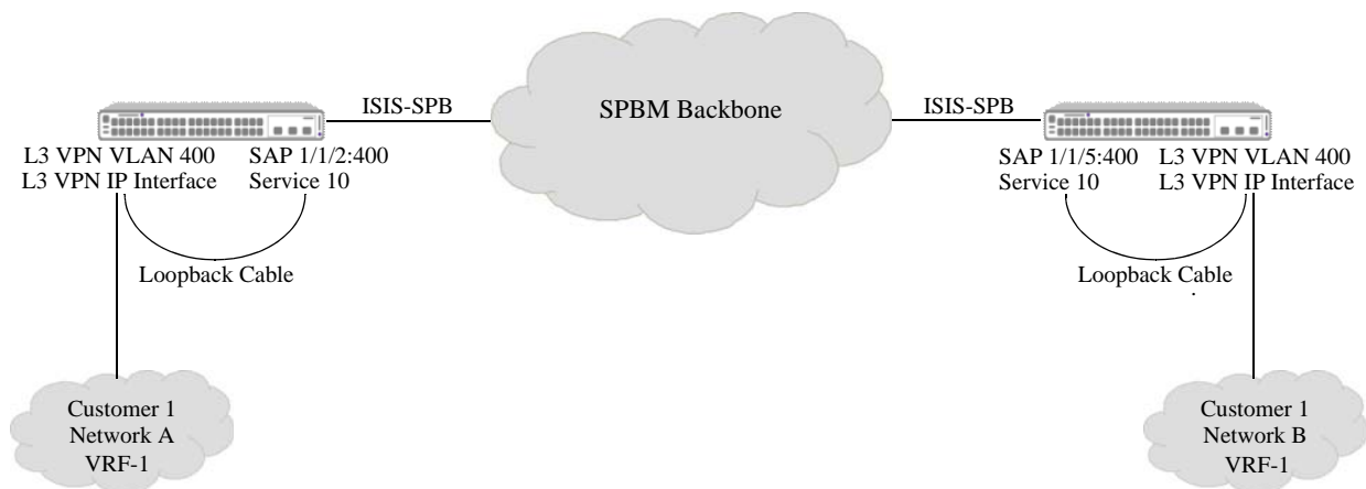
Figure 9: L3 VPN Interface: External Loopback
