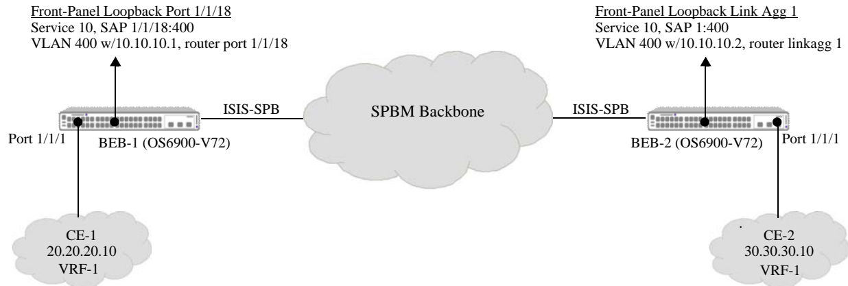
Figure 12: L3 VPN Front-Panel Ports (In-Line Routing)
