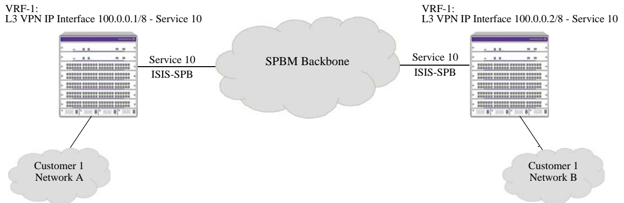
Figure 7: L3 VPN Interface: In-line Routing (OmniSwitch 9900)
