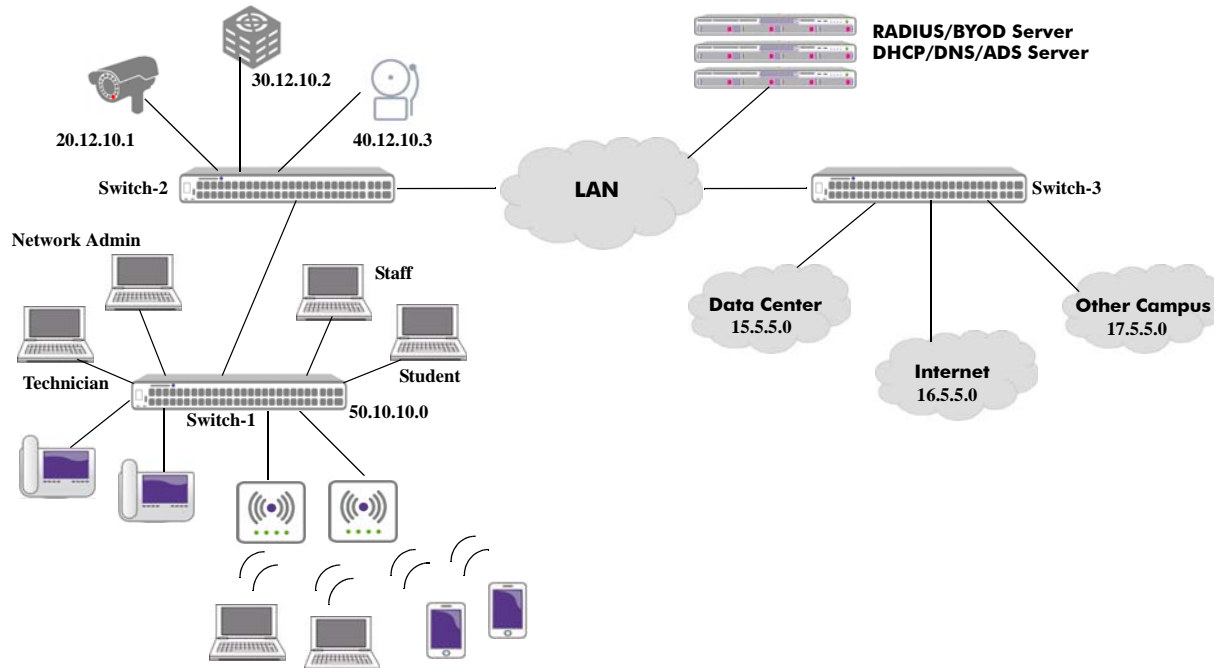
Campus Network Topology Example
