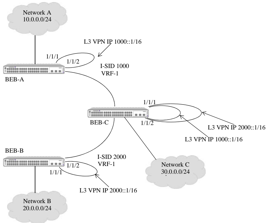
Figure 15: IPv6 Inter-ISID Routing Example (One VRF)
