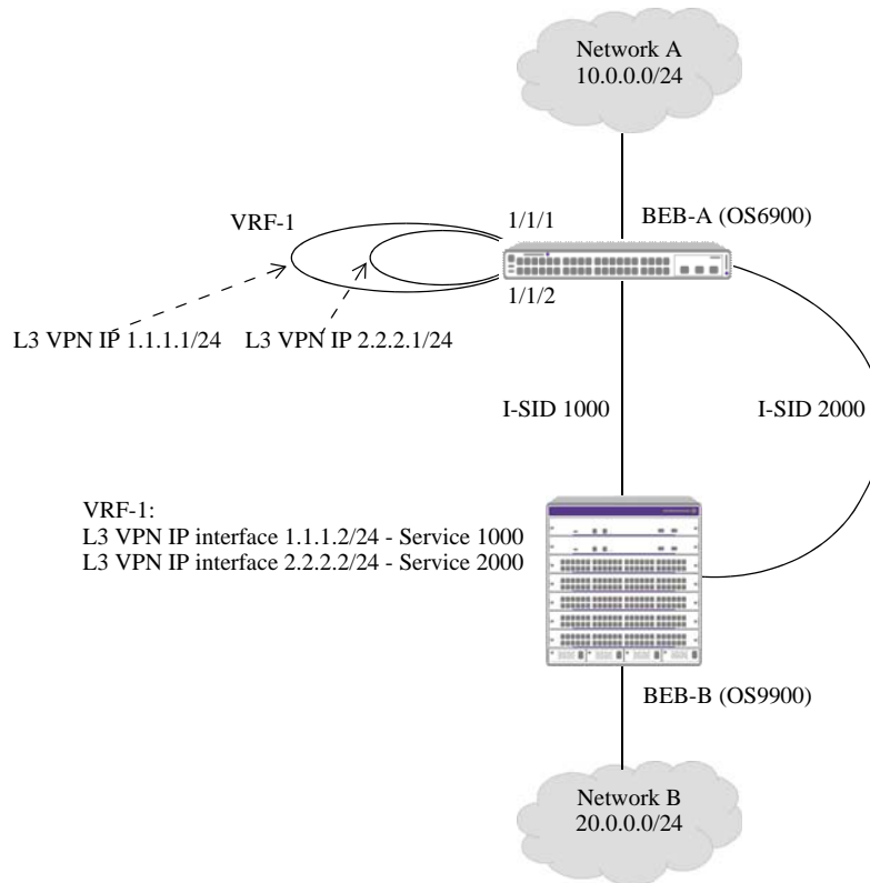
Figure 13: IPv4 L3 VPN External Loopback and Service-based Interfaces
