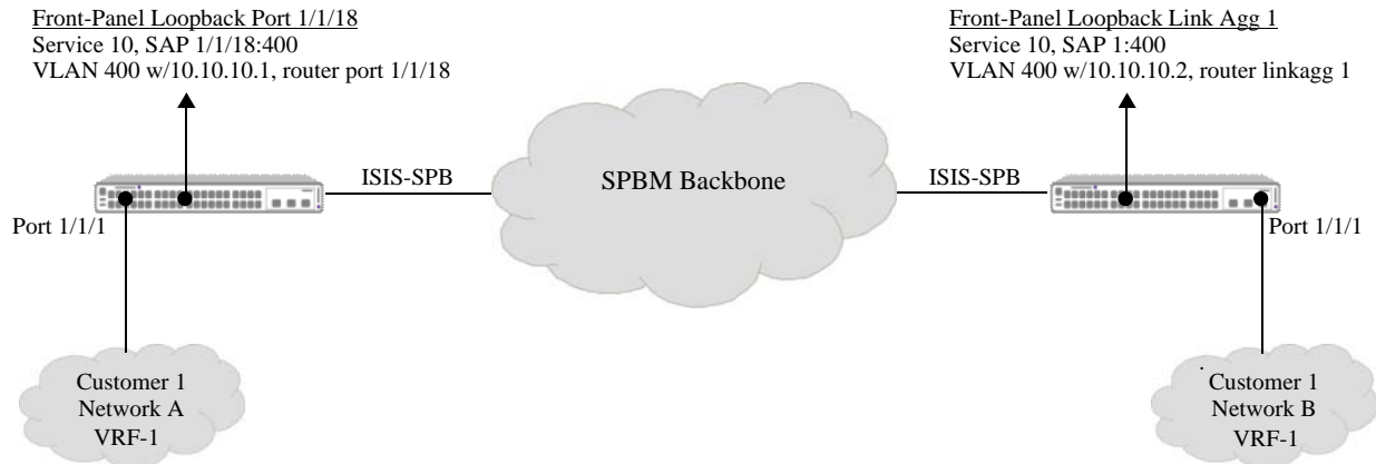
Figure 8: L3 VPN Interface: Inline Routing (OmniSwitch 6900-V72, 6900-C32)
